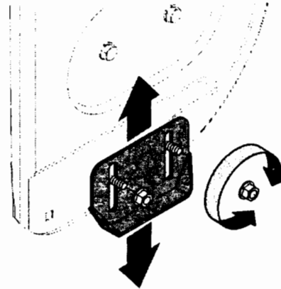
Figure 19- Patin ordinaire
